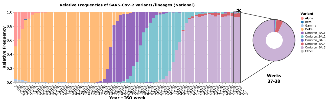
Figure 1: Evolution of the weekly relative frequency of the SARS-CoV-2 variants circulating in Portugal between ISO weeks 22 (31/05/21 - 06/06/21) and 38 (19/09/22 - 25/09/22). The frequencies presented for the last week under analysis (ISO week 38*) might change in the next report, given that some data from that period is still being processed. This and other graphs can be explored interactively on the website.
